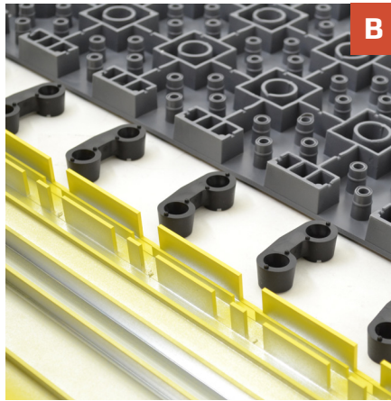
Use LockSafe® connectors to join males on ramps to males on ErgoDeck® tiles
