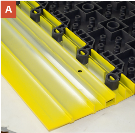
Connect males on ramps to females on ErgoDeck® tiles
